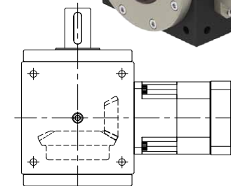
R 軸 Shaft Direction
